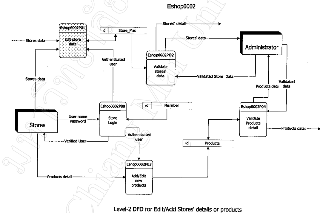
Level-2 DFD for Edit/Add Stores' details or products
