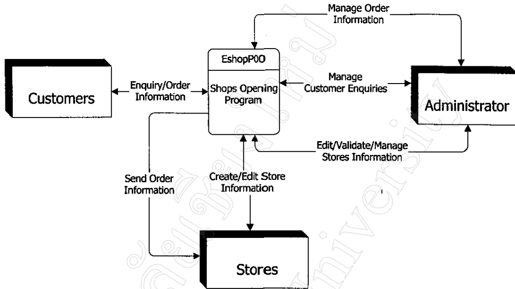
Level-0 Opening Shop System Context-level DFD
