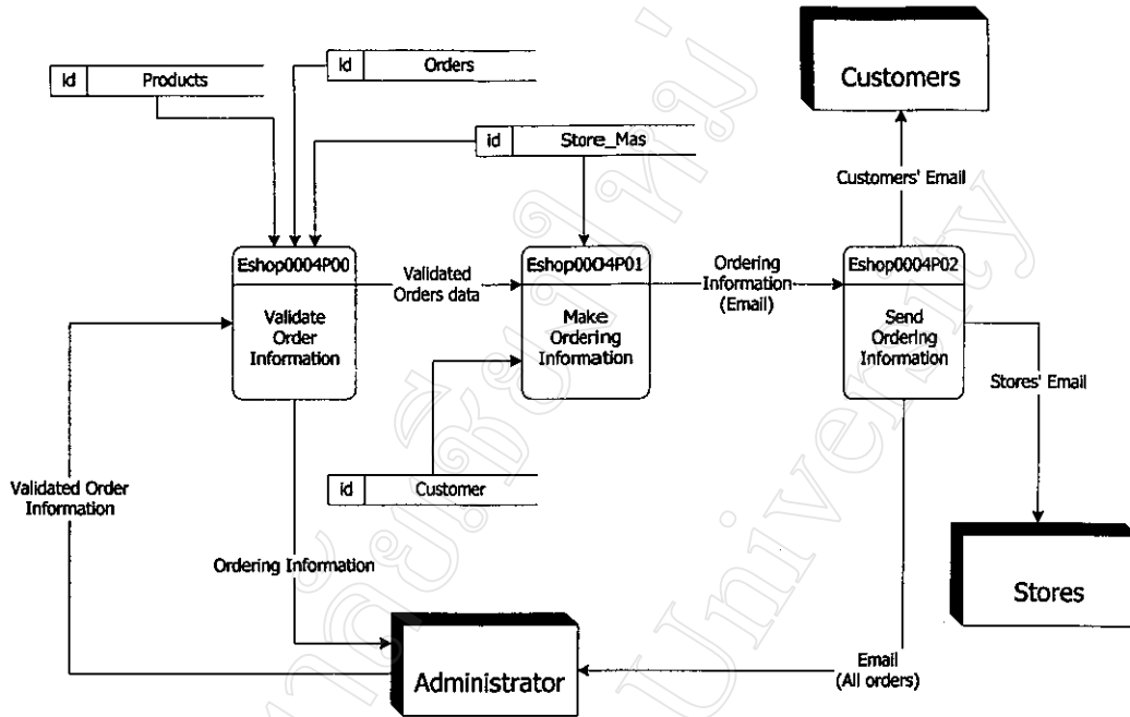
Level-2 DFD for Validate/Manage Orders Information
