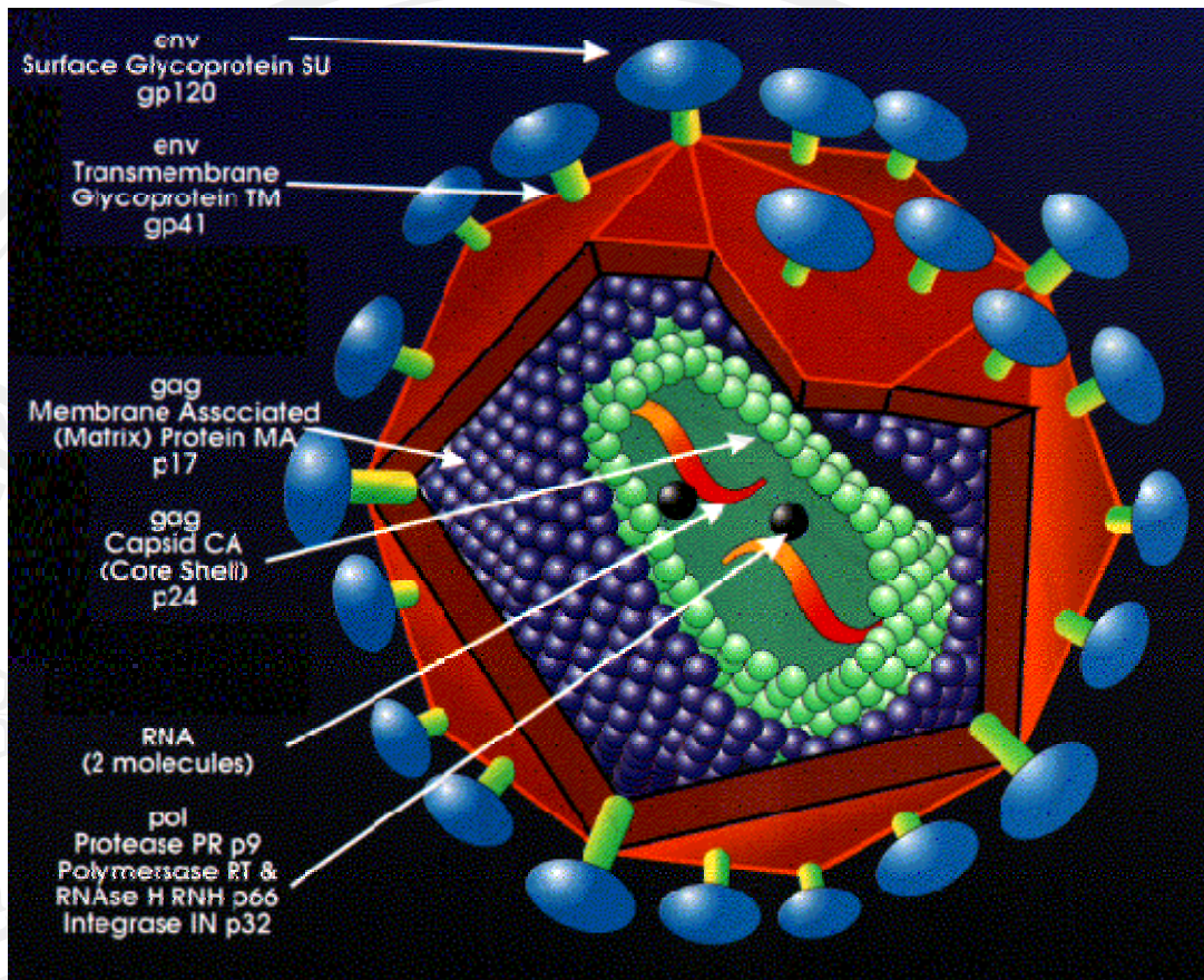
Figure 1.1 The structure of human immunodeficiency virus (HIV).
