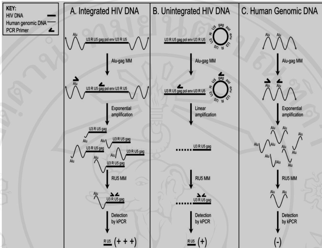
Figure 1.10 An overview of Alu-gag qPCR assay (Liszewski et al., 2009).
