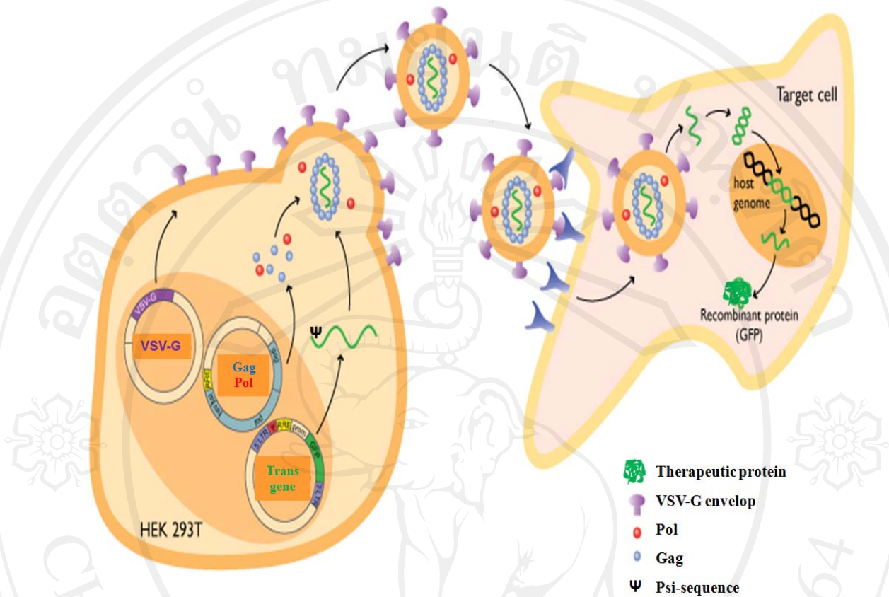
Figure 1.15 The overall picture of lentiviral gene therapy. (Adapted from http://www.invivogen.com/sscat.php?ID=116&ID_cat=16 ) Transfer vector is flanked by LTRs and the Psi-sequence ( \Psi ) of HIV. This vector is transfected or cotransfected with packaging plasmids into a packaging cell line which can produce viral proteins to form virus shell. The RNA of transgene is packed into virion. This virion contains only RNA of transgene without sequences of viral components. Therefore, it lack of responsibility of replication after they deliver their therapeutic transgene. RNA transgene is reversed into double-stranded DNA by RT and is integrated into a host genome by IN. Then, translation occurs to produce therapeutic protein.
